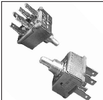
Chalk's Part #: CSB-508 5 Blade, Twist, Heater Switch, 5/16\" Long (Blue Bird), 3 Speed Knobs: 28-51601 (Butterfly), Snowflake 28-51602 (Round), Fan 29-21905 Longer Shank (5/8\") 33-41431 Pigtail, 5 Wire
