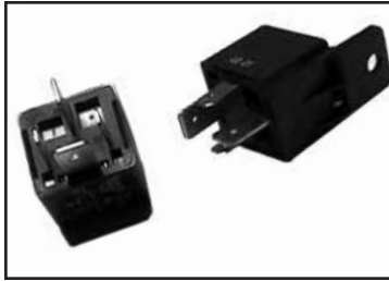
Chalk's Part #: 30-13420 Relay, 2 Large Blades, 2 Small Blades, 70AMP 4 Blade
