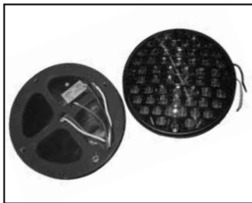
Chalk's Part #: 756-IRRDR 7" Warn 56 LED , Strobing, Red Lenses, 3 Wire, SoundOff
