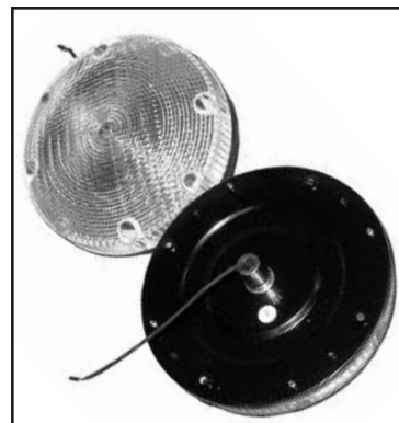
Chalk's Part #: 1010CS 7" Back Up Light, Socket Back, Clear, Weldon Bulb #: 1156 Lens #: 1003-0000-30 1010CF Clear-Flat Back
