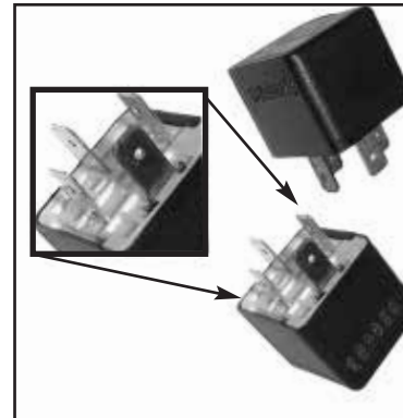
Chalk's Part #: 30-13399 Bosch A/C Delco Relay 12V 40 Amp, 4 Blade,
