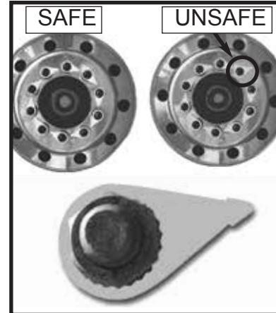
Chalk's Part #: WLCH-B - 33MM WLCH-AA - 1 1/2" Wheel Check, Other Sizes Available (Visual Check For Loose Nuts )
