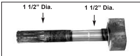
Chalk's Part #: CS41017 S-Cam, We Have All The Cams. S-Cams, 1 1/4", 1 1/2", 1 5/8"; Various Lengths. Front & Rear To Order We Need: 1 Is It Right Hand Or Left 2 Diameter (1 1/4" - 1 1/2") 3 Length From Under Head To End 4 Number Of Splines
