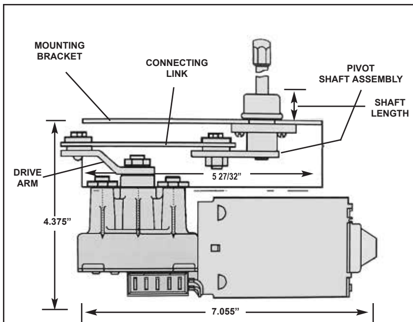
Typical Illustration of Wiper Motor Mounting
