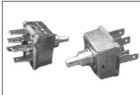
Chalk's Part #: CSB-508 5 Blade Rotary AC-Heater Switch, 5/16" Short Threaded Shaft
