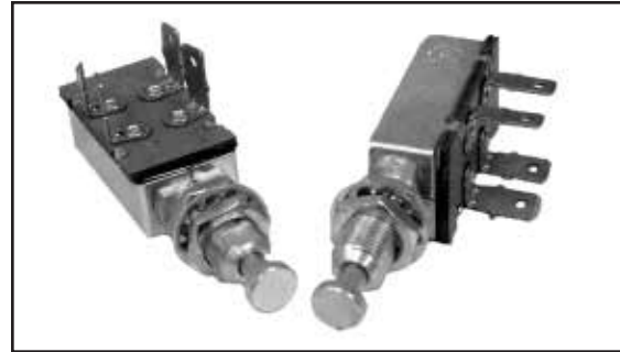
Chalk's Part #: S154 Door Switch, Normally ON, OFF When Plunger Depressed, 4 Blade
