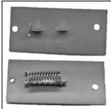
Chalk's Part #: CSB-505 Wayne, Heater Resister, Single Coil, 3 Blades
