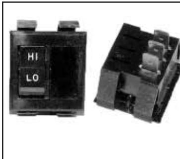
Chalk's Part #: R360 3 Position One Side Blank One Side HIGH-OFF-LOW, 3 Blade
